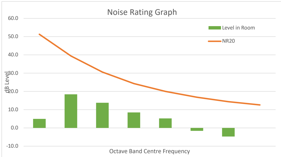
Figure 2: Predicted NR curve against NR20
